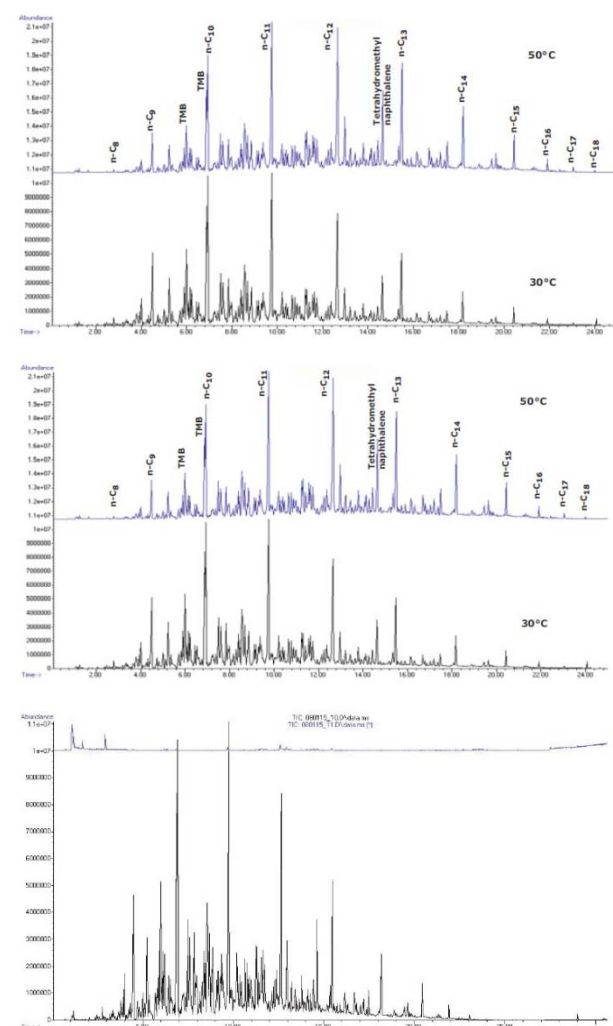
Figure 2. Top: Diesel vapor collected from dry sand samples at 30°C and 50°C using soil gas tubes. Middle: Diesel vapor collected from wet sand samples at 30°C and 50°C using soil gas tubes. Bottom: Diesel vapor analysis with repeat desorption of tube showing negligible carryover.
