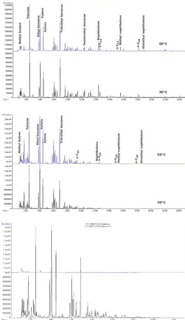
Figure 1. Top: Gasoline vapor collected from dry sand samples at 30°C and 50°C using soil gas tubes. Middle: Gasoline vapor collected from wet sand samples at 30°C and 50°C using soil gas tubes. Bottom: Gasoline vapor analysis with repeat desorption of tube showing negligible carryover.
